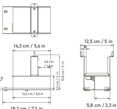
Canaleta media / Middle channel
