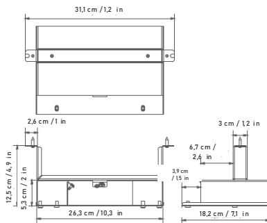
Unión canaleta perimetral media / Middle perimeter channel joint
