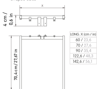
Base rectangular en U / Rectangular U-shaped base
