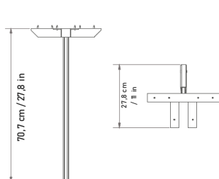
Base pedestal / Pedestal base
