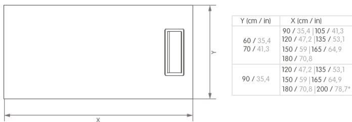
Superficies electrificación lateral/ Side electrification surfaces
