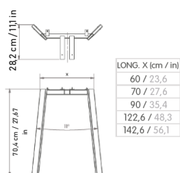
Base trapezoidal / Trapezoidal base
