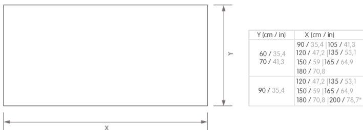
Superficies recta lisa / Smooth straight surface
