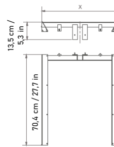
Base triangular en U / U-shaped triangular base
