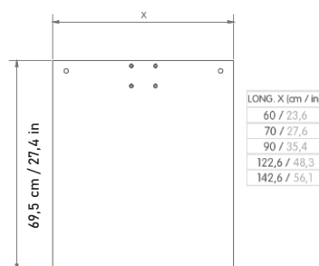
Base madera / Wooden base
