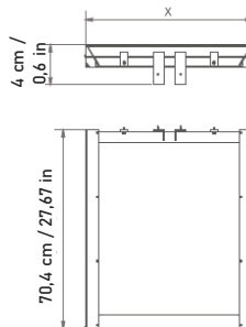
Base triangular en marco / Triangular base in frame
