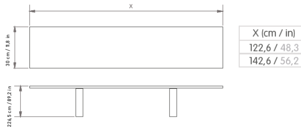
Superficies counter / Counter surfaces
