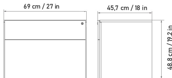
Archivador 1x1 spine 70 / 1x1 cabinet, spine 70
