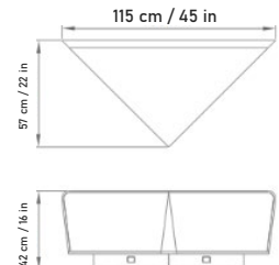
Conector 90° / 90° connector
