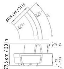
Asiento curvo / Curve seat module
