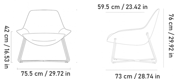
Base trineo / Sled base
